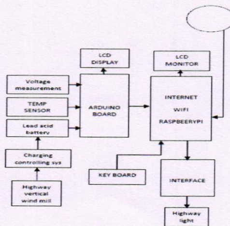
Fig.1: Block diagram of proposed work
