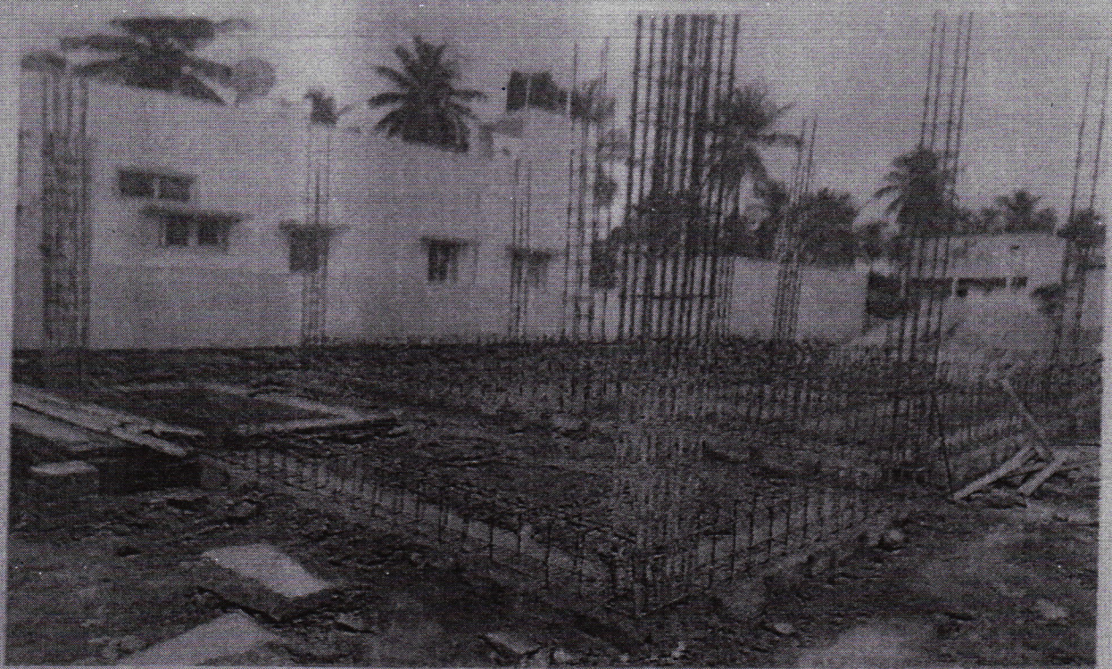
Fig 9: Plinth beams
