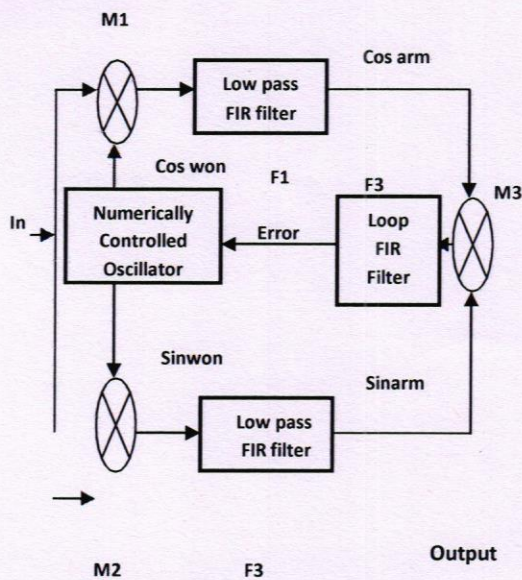
Fig.1 Block diagram Costas loop
